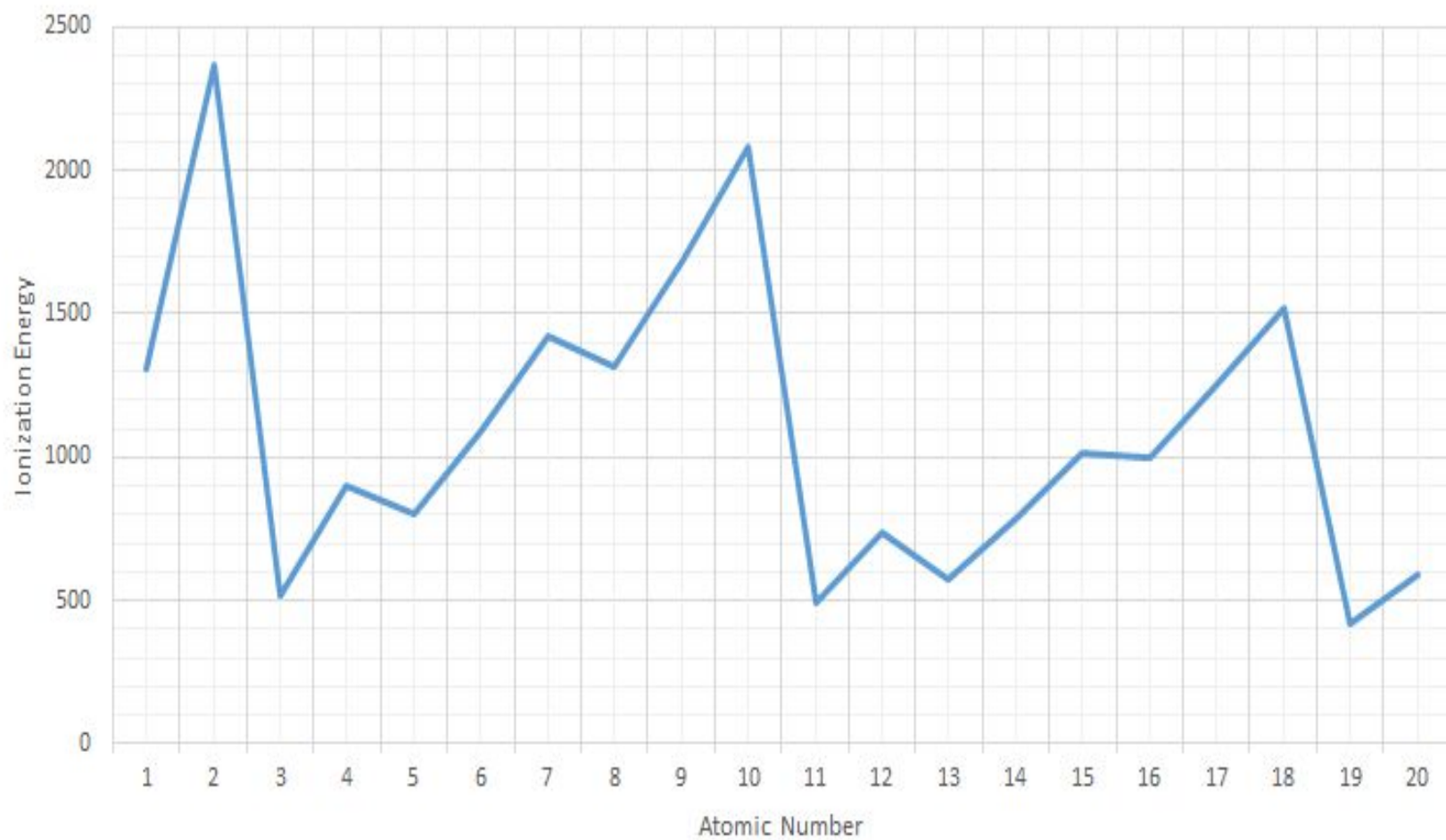
Ionization Energy versus Atomic Number for the Elements of the Periodic Table
